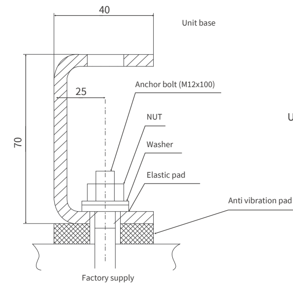
Detailed drawing of foundation installation (not to scale)
